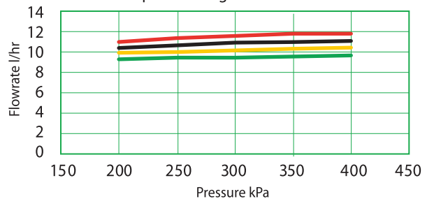
Radius Chart of the pressure regulated RC 007-PR
